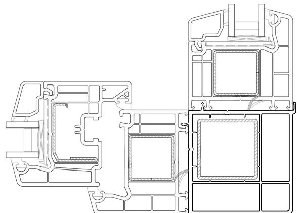
Corner Casing
