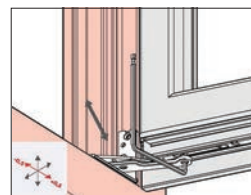
Gasket-compression adjustment pivot rest
