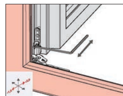
Lateral adjustment corner hinge
