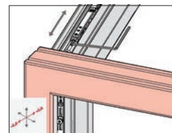
Lateral Adjustment sash stay
