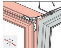
Gasket-compression adjustment sash stay
